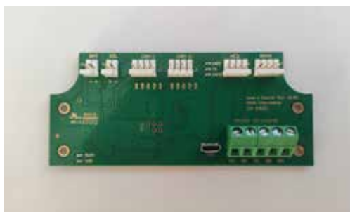
Control Unit Board
