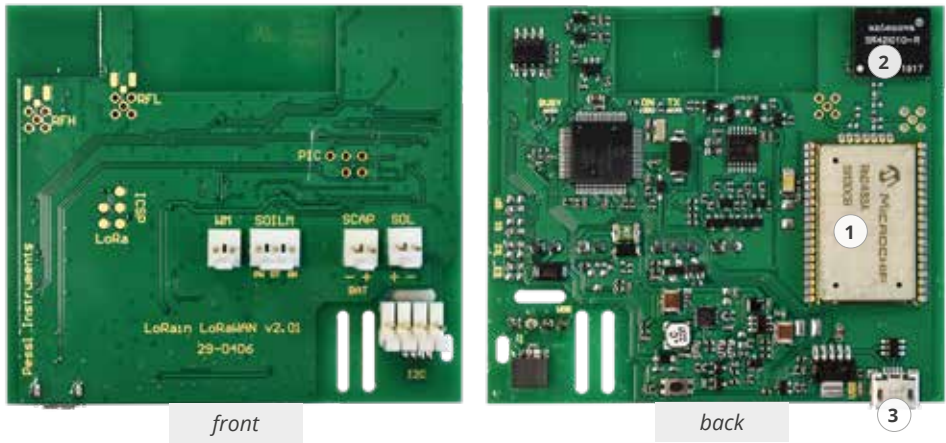
LoRAIN and LoRATH LoRa gen 3 (29-0406)
