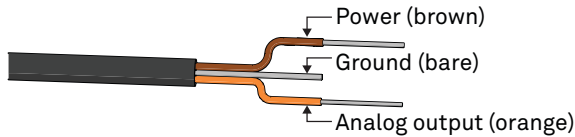
Figure 2 Pigtail wiring
