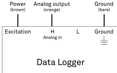
Figure 3 Wiring diagram
